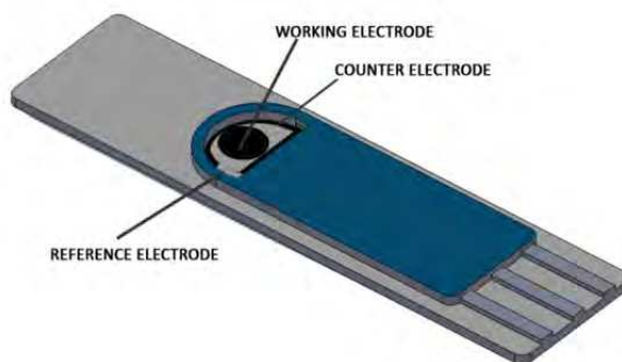
Fig. 3. Electrochemical biosensor as screen printed electrode.
