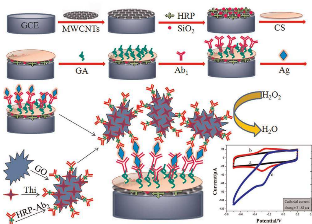
Fig 2. Schematic process of preparing modified electrode by encapsulation of enzyme in silica matrix. This figure was obtained with permission from Ref [40]
