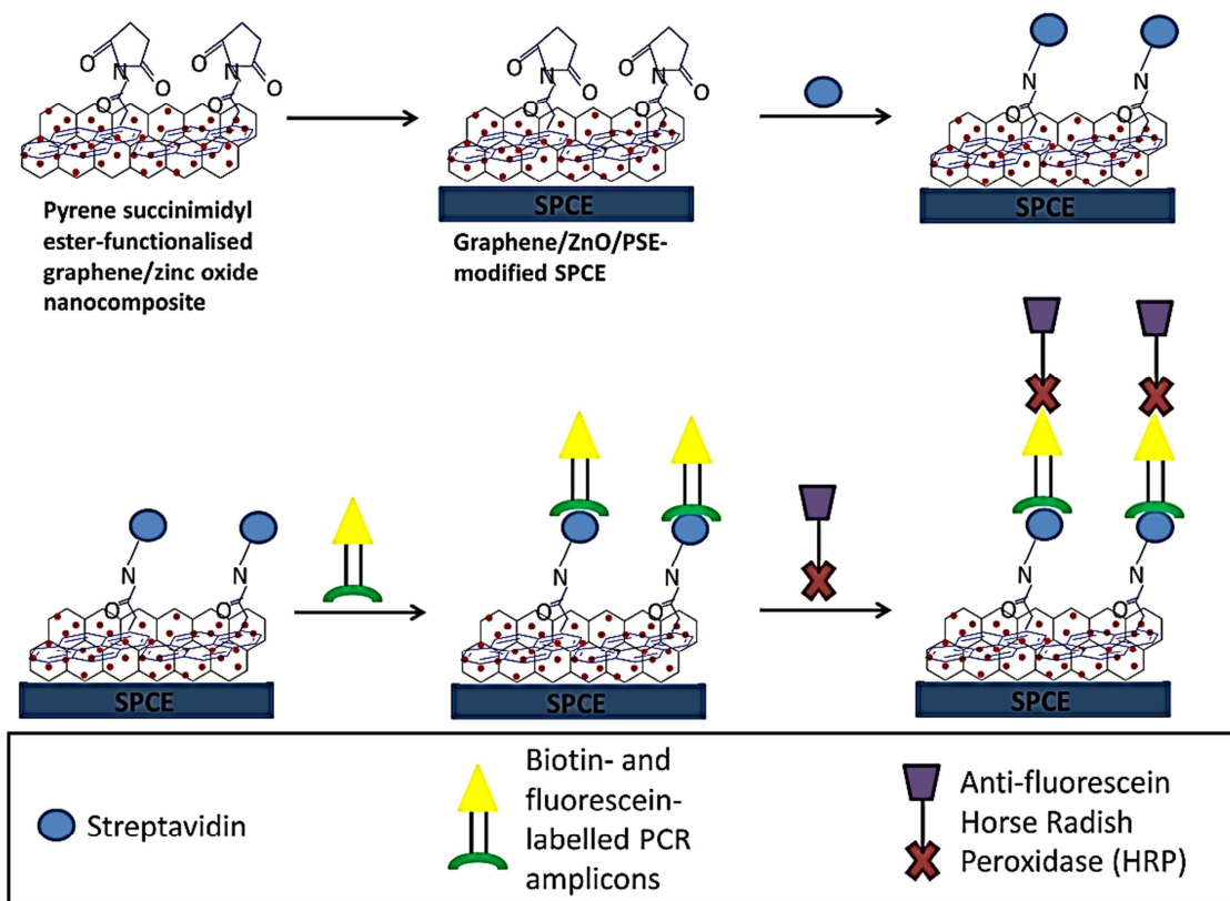
Fig 6. Preparation of a biosensor based on graphene/zinc oxide nanocomposite and its application in detection of Influenza H5 gene. This figure was obtained with permission from Ref [86].
