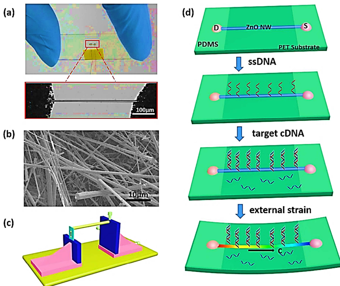
Fig 5. ZnO nanowire-based biosensor for detection of human immunodeficiency virus (HIV) (a) Digital and microscopy image of ZnO nanowire DNA sensor. (b) SEM image of ZnO nanowires. (c) schematic explanation of biosensor design. (d) performance of ZnO nanowire DNA sensor regarding external strains. This figure was obtained with permission from Ref [85]
