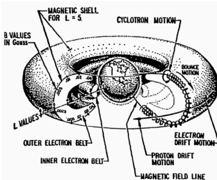
Charged Particle Motion in Earth's Geomagnetic Field
