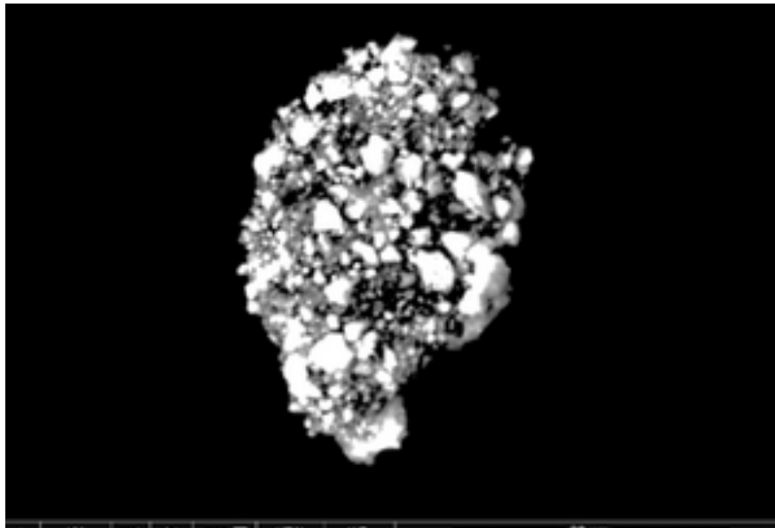
[Figure 22 A Stainless Steel Aggregation of Carbon , Oxygen, Iron and Nickel Held Together With Graphene Oxide.[75]]
