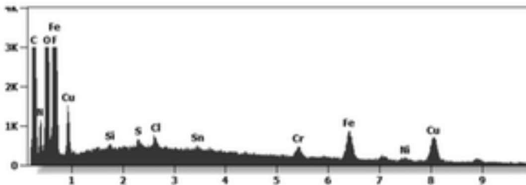
[Figure 19 - Engineered aggregate of iron, chromium and nickel also know as stainless steel.[75]]
