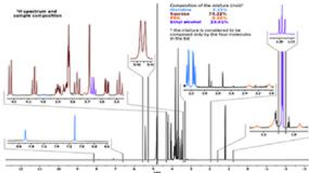
[Figure 21 Identifies the Spectrum of AstraZeneca Vaccine Adjuvants. Different colors are used for the four molecules identified by means of reference spectra. Relative concentration is calculated on integrals of reference signals for molecules in a quantitative spectrum acquired with a duty cycle of 5 seconds with the longest calculated T1 was 5sec.]
