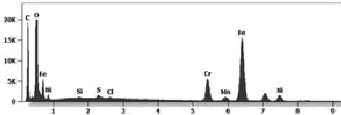
[Figure 23 Shows Elements of Carbon , Oxygen, Iron and Nickel Held Together With Graphene Oxide.[75][83]]
